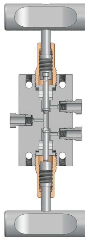
Diverter 2 (1 Inlet Port)
