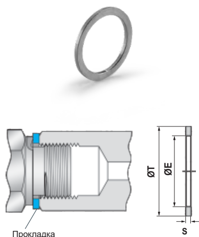
ISO PRP Gaskets For Parallel Threads
