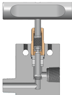
2-Way Straight Male to Female NPT
