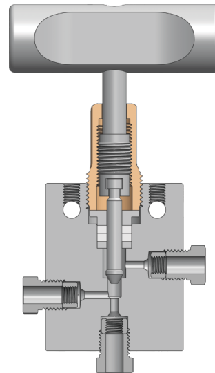
Diverter 2 (1 Inlet Port)
