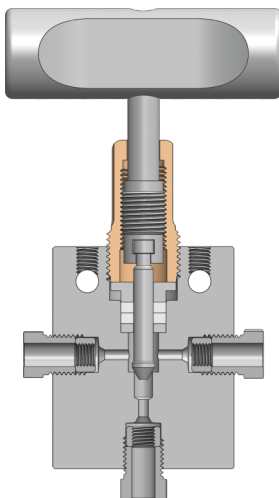
Diverter (2 Outlet Ports)
