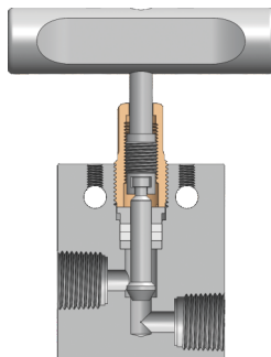
2-Way Straight Female to Female NPT
