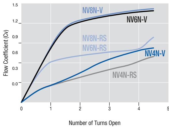
15000 psi (1034 bar) Pressure Rating
