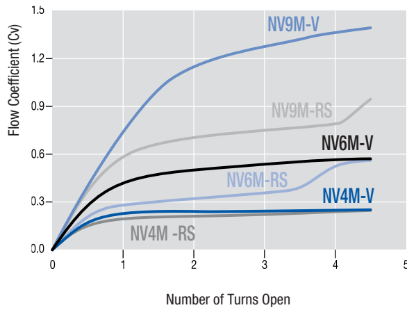
20000 psi (1378 bar) Pressure Rating
