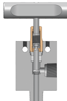
2-Way Angle Male to Female NPT
